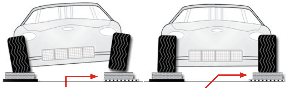
See how the LF pad slides sideways, relieving camber bind.
